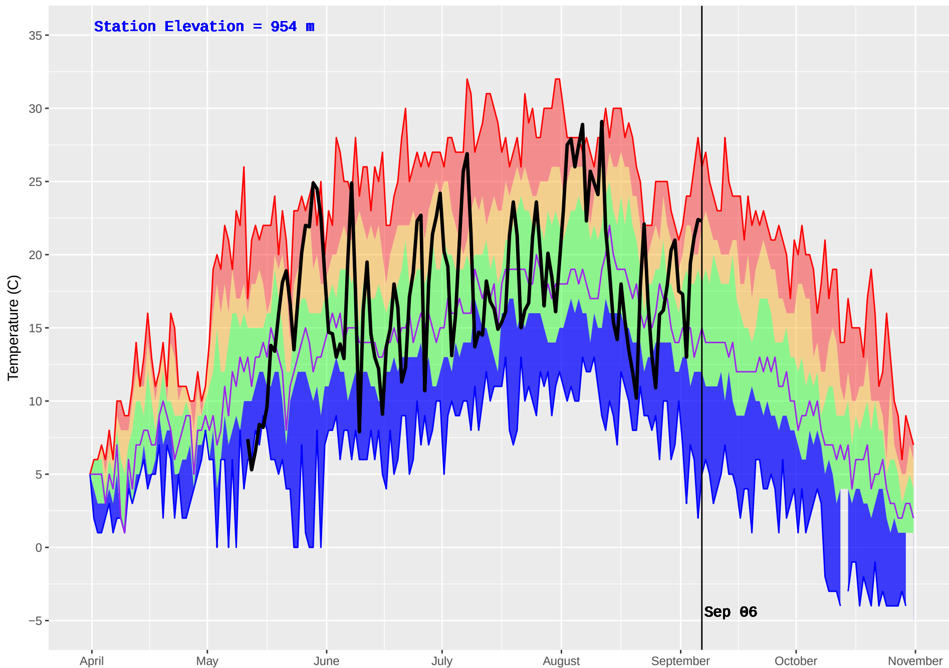
NADINA (179) : Historical (1985–2016) and Current (2017) Noon Temperature
