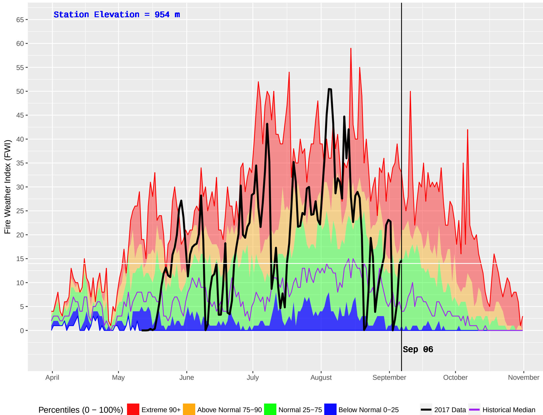
NADINA (179) : Historical (1985–2016) and Current (2017) Noon Fire Weather Index (FWI)
