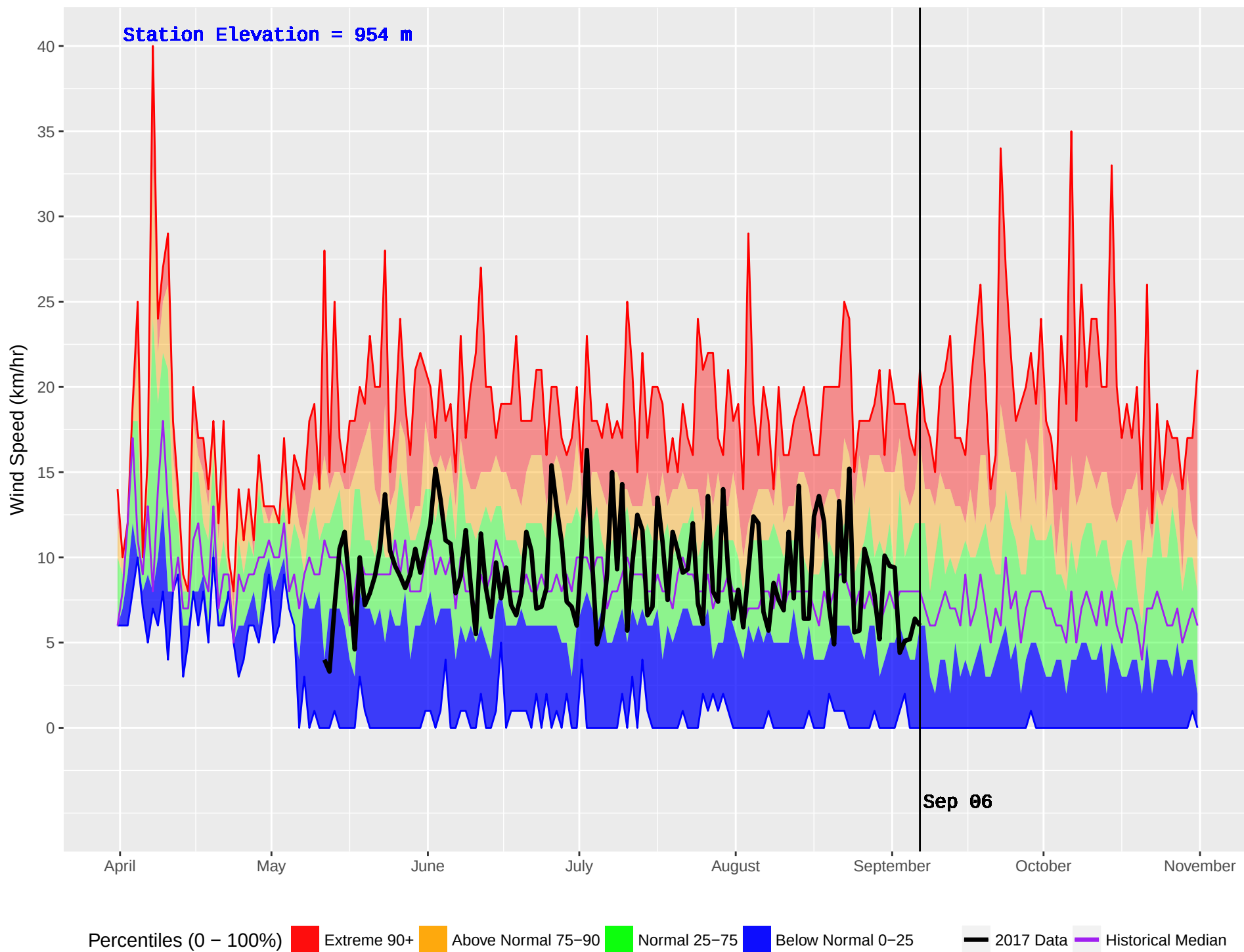
NADINA (179) : Historical (1985–2016) and Current (2017) Noon Wind Speed
